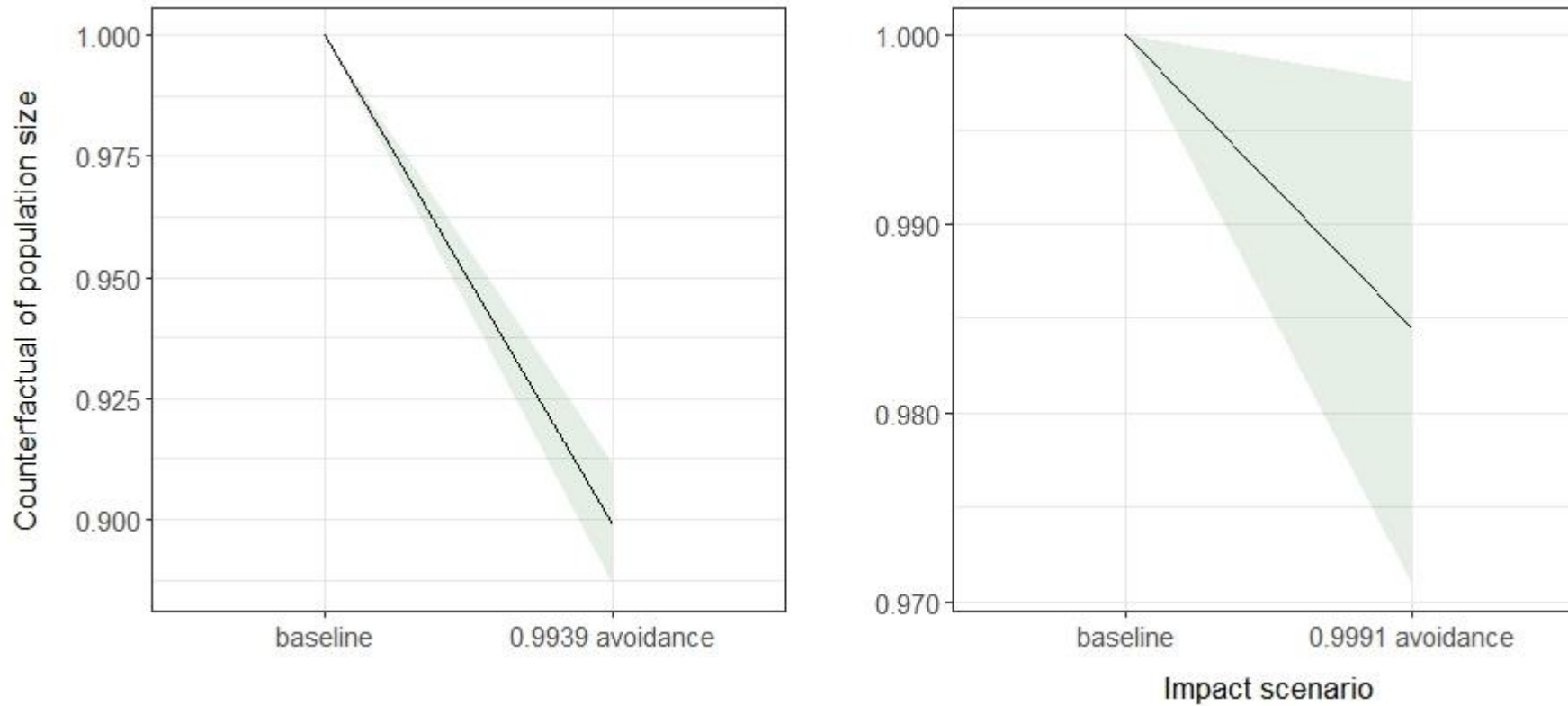
Figure 1.15: The ratio of the median impacted annual population sizes for the South-West and English Channel BDMPs using grouped avoidance rates (0.9939) and species-specific avoidance rates (0.9991) from the simulations after 35 years.
