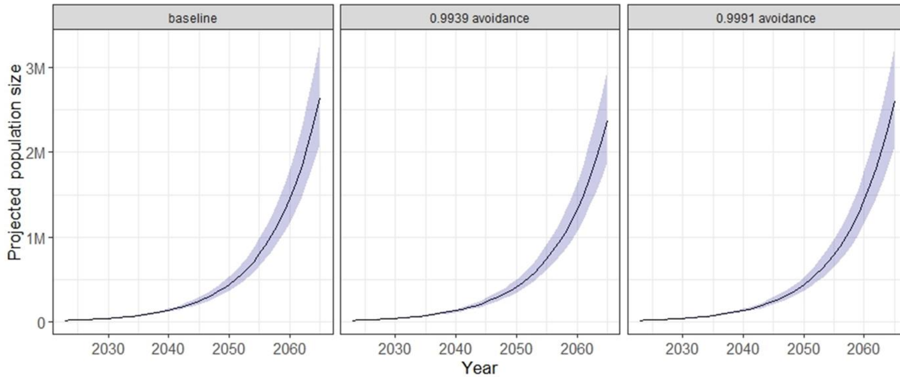
Figure 1.13: Projections of population sizes over a 35-year time-frame for the South-West and English Channel BDMPS using JNCC avoidance rates. Each plot represents a different impact scenario in terms of additional adult mortalities (starting at baseline (i.e. unimpacted)).
