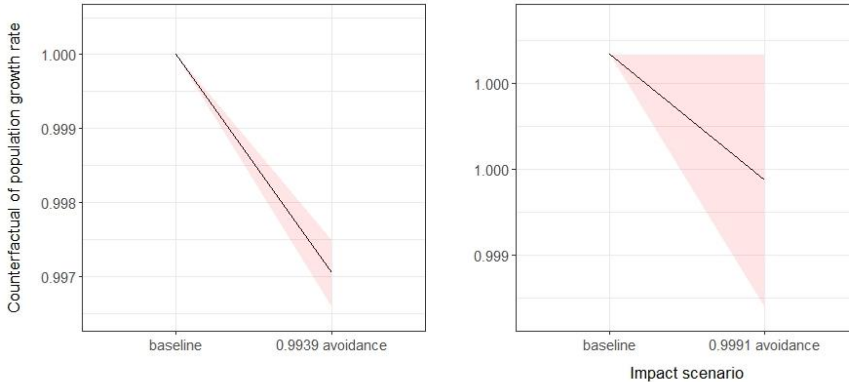
Figure 1.14: Ratio of annual impacted growth rates after 35 years for the South-West and English Channel BDMPS using grouped avoidance rates (0.9939) and species-specific avoidance rates (0.9991).
