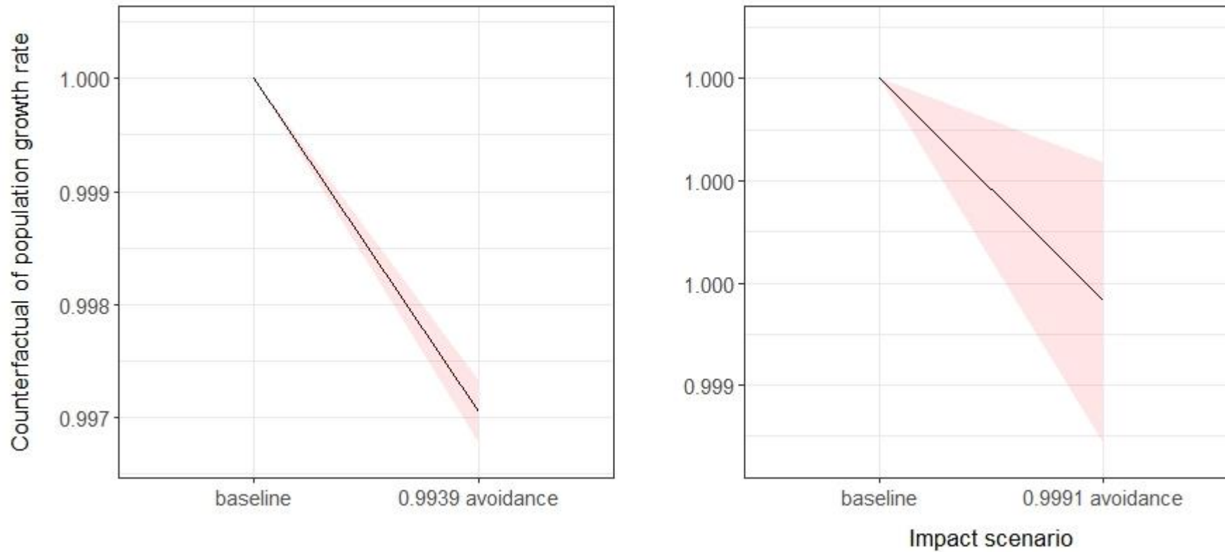
Figure 1.11: Ratio of annual impacted growth rates after 35 years for the South-West and English Channel BDMPS using species-group avoidance rate (0.9939) and species-specific avoidance rate (0.9991).
