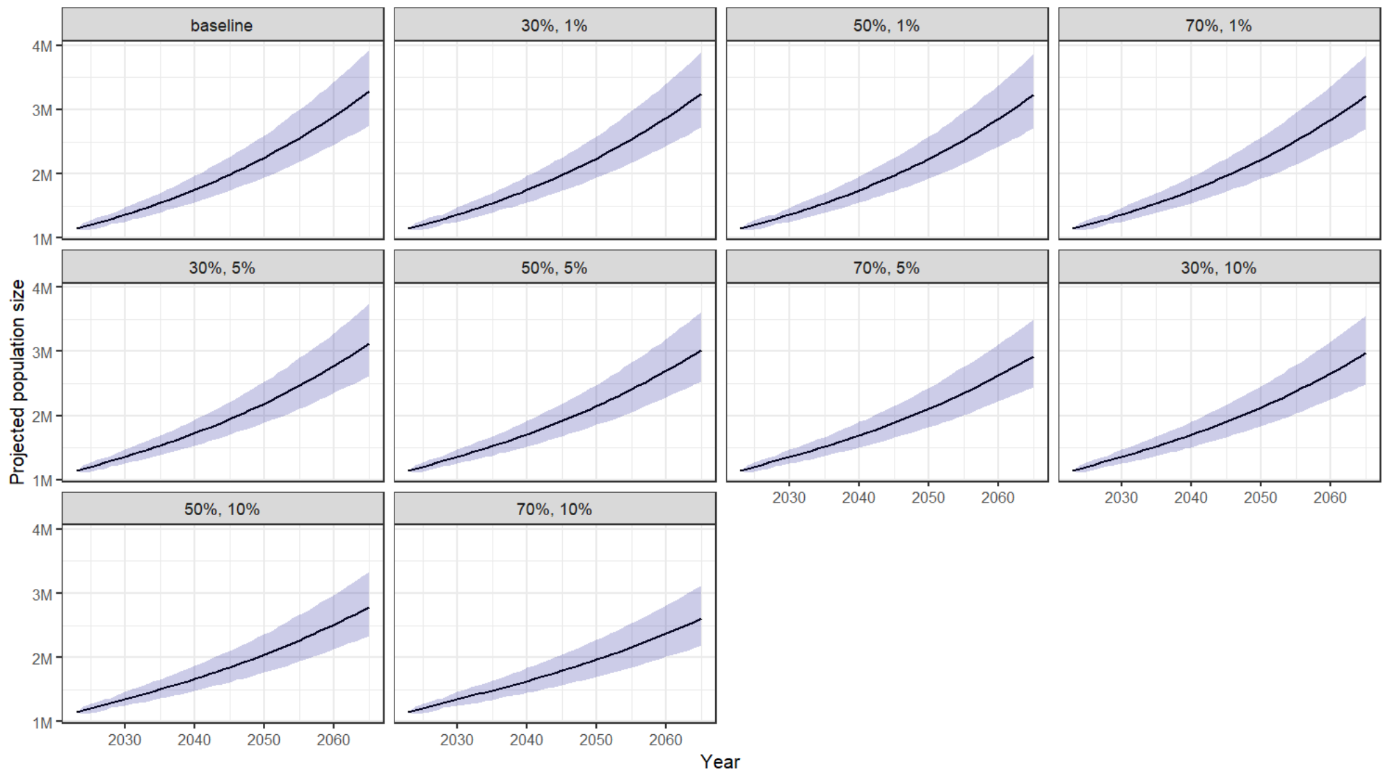
Figure 1.7: Projections of population sizes over a 35-year time-frame for the UK Western waters BDMPS. Each plot represents a different impact scenario in terms of additional mortalities (starting at baseline (i.e. unimpacted))
