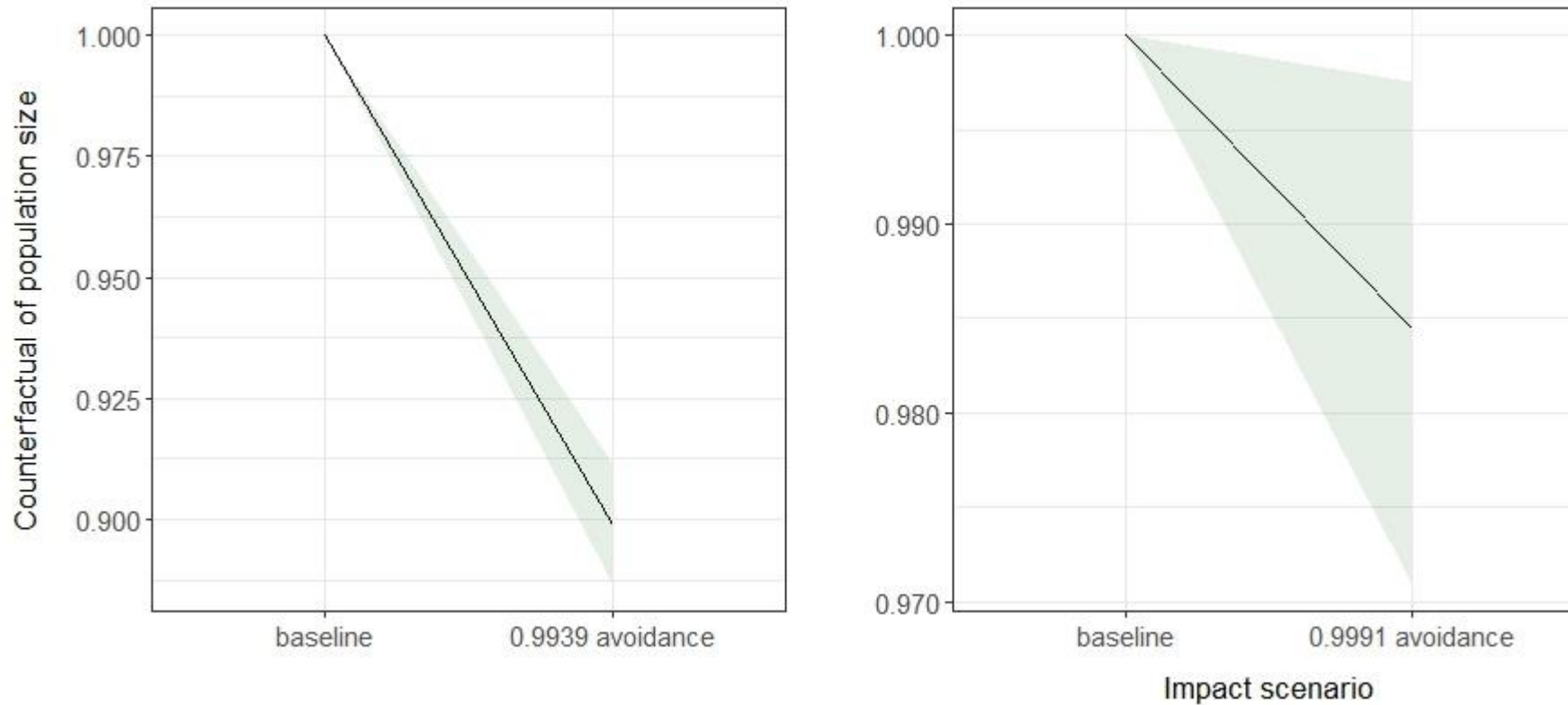
Figure 1.12: The ratio of the median impacted annual population sizes for the South-West and English Channel BDMPS using species-group avoidance rate (0.9939) and species-specific avoidance rate (0.9991) from the simulations after 35 years.
