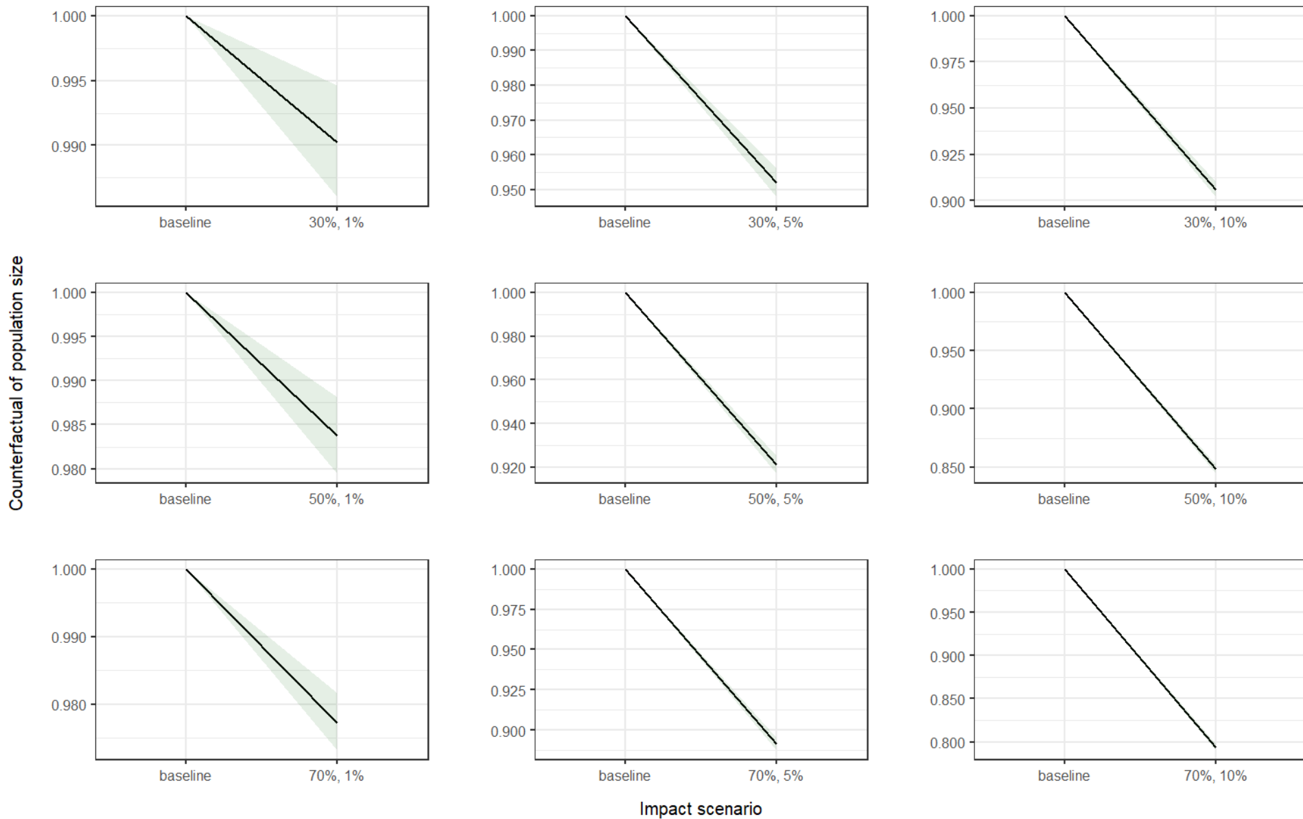
Figure 1.9: The ratio of the median impacted population sizes for the UK Western waters BDMPs under a range of impact scenarios after 35 years.
