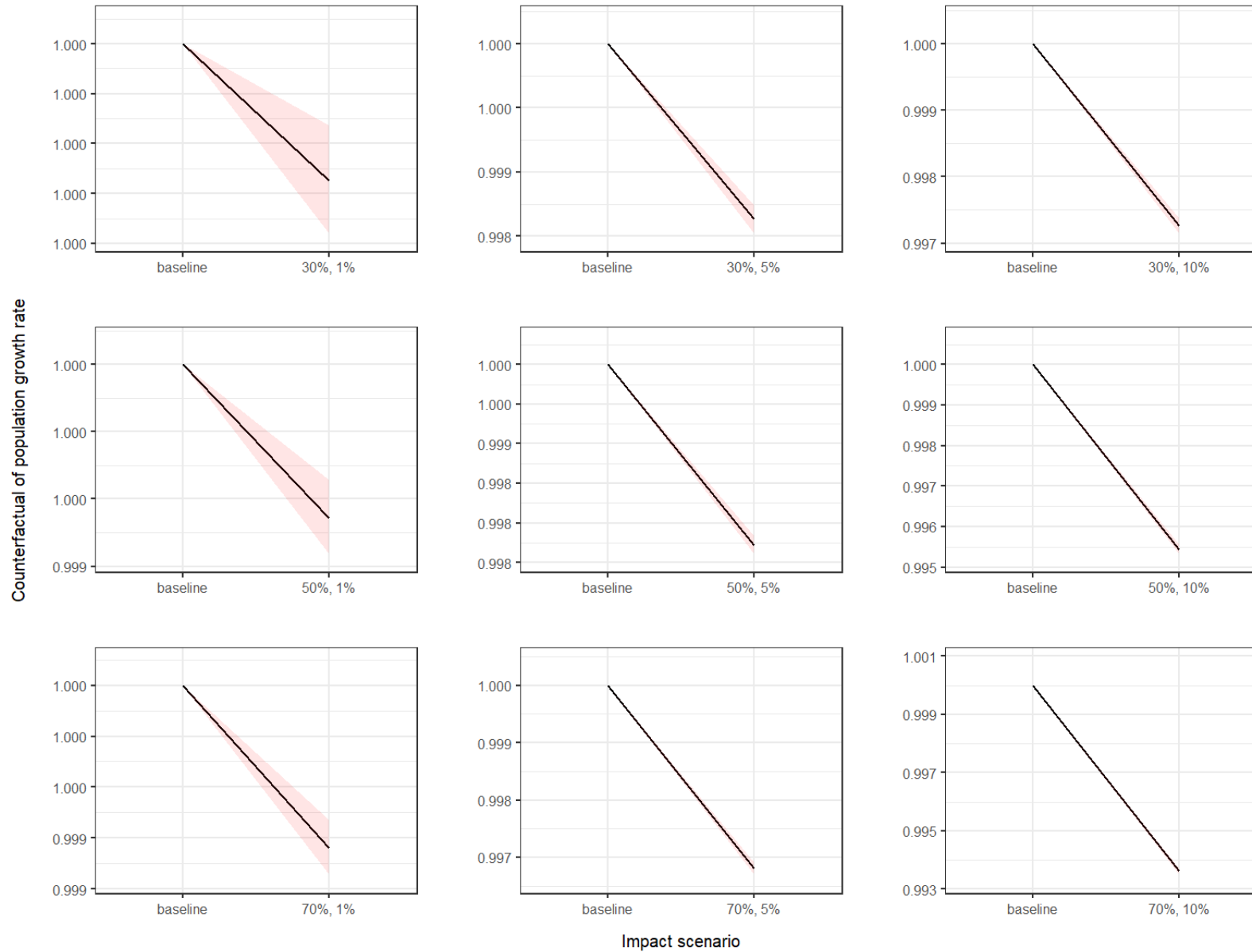
Figure 1.8: Ratio of impacted growth rates after 35 years for the UK Western waters BDMPS under a range of impact scenarios after 35 years.
